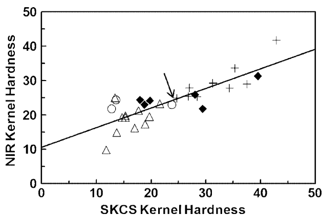
Figure 1. SKCS kernel hardness versus NIR kernel hardness for 30 eastern and western US soft wheat cultivars grown in Washington state. Each data point is the mean of 12 observations (2 replicates \times 2 sites \times 3 years); 'plus' = soft white Club, 'triangle' = soft red winter, 'circle' = eastern soft white winter, and 'diamond' = western soft white wheat cultivars. The arrow indicates the separation point of eastern cultivars from Club cultivars.
